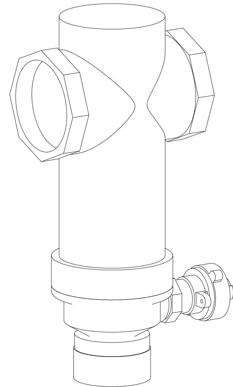
Isometric view
