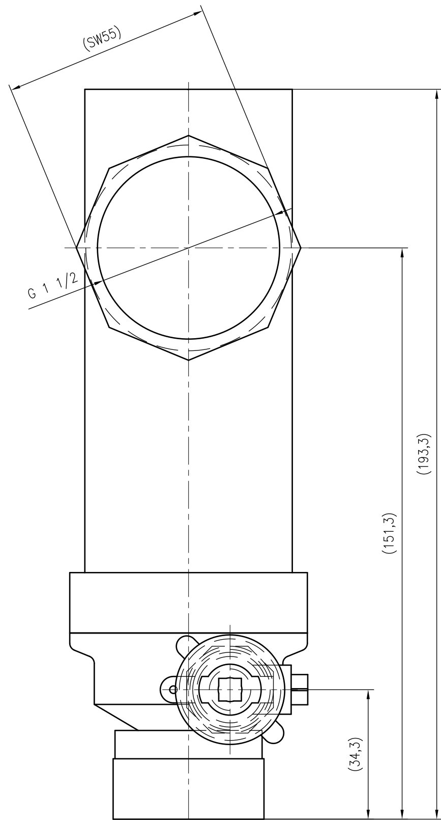
Side view
