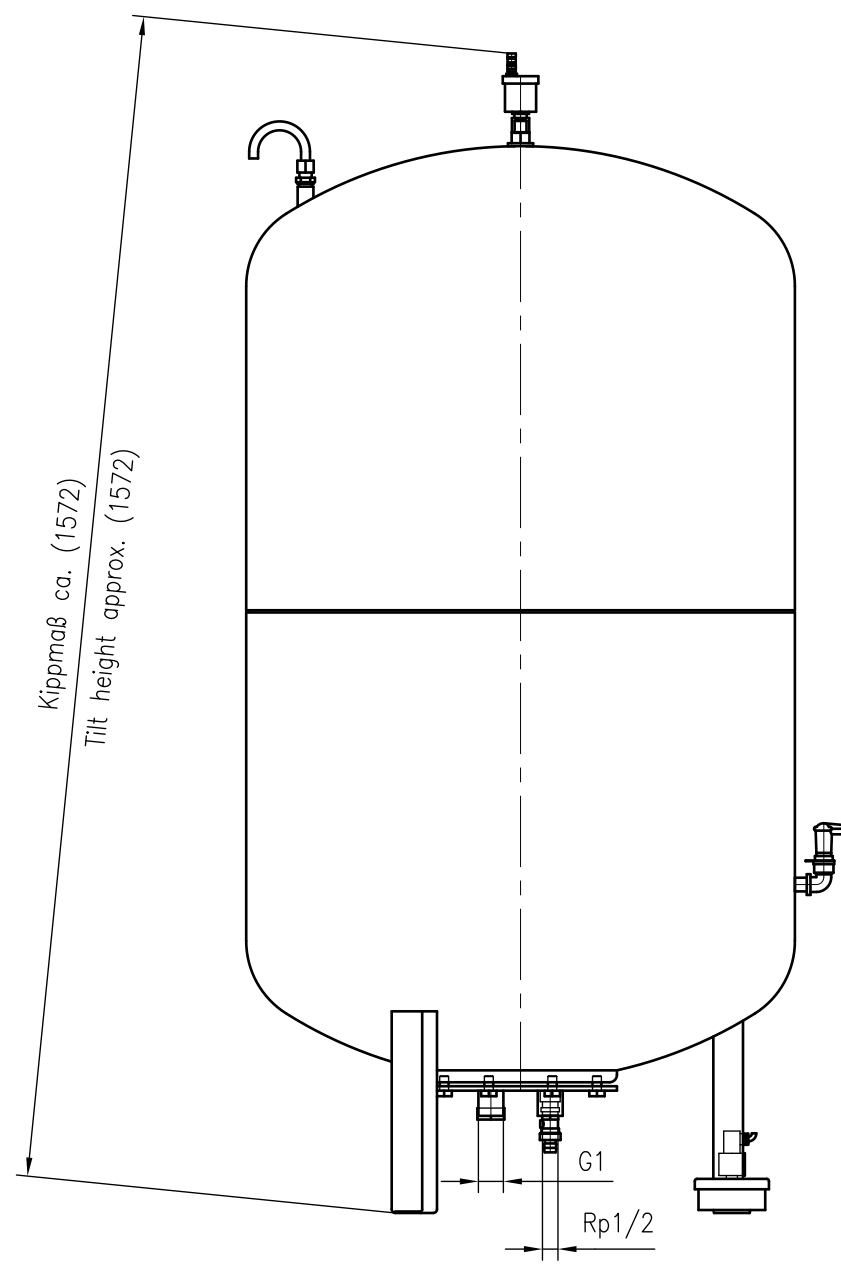
Side view
