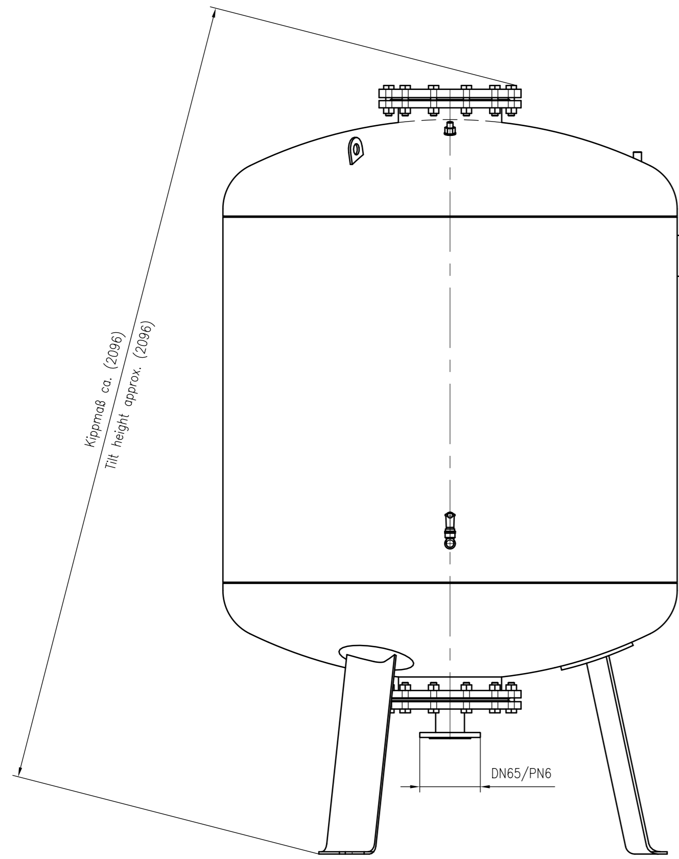
Side view
