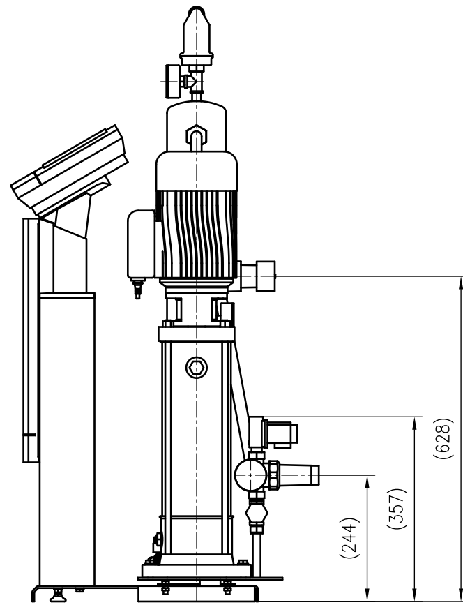
Side view
