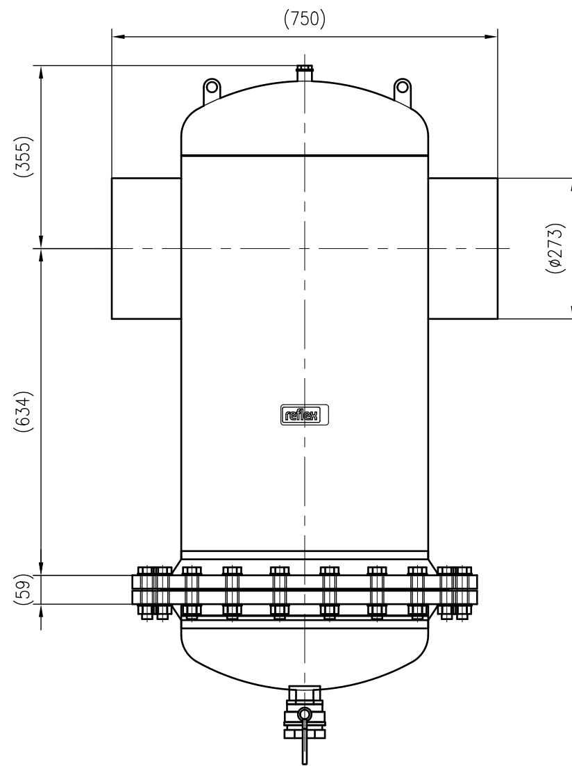
Front view
