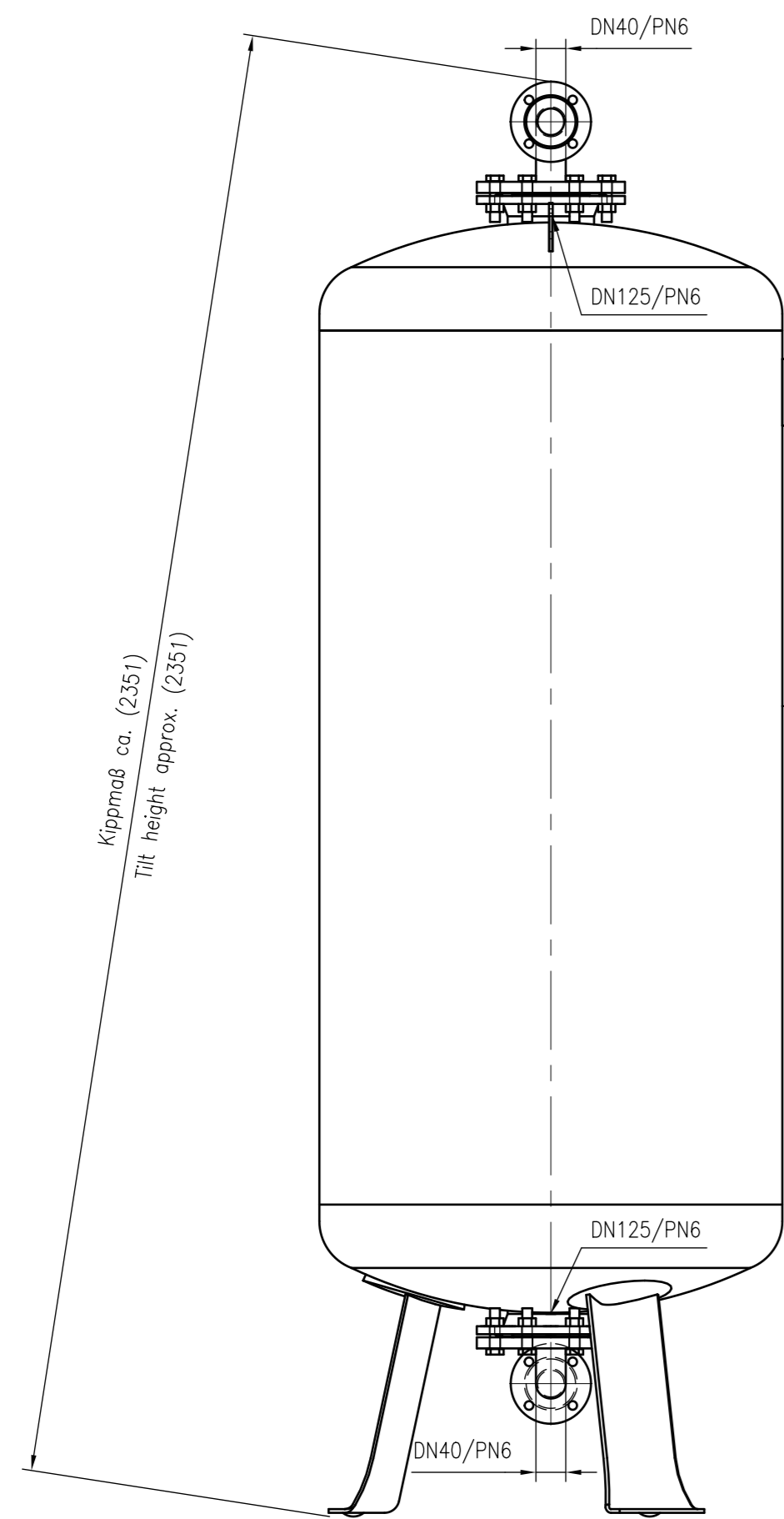
Side view
