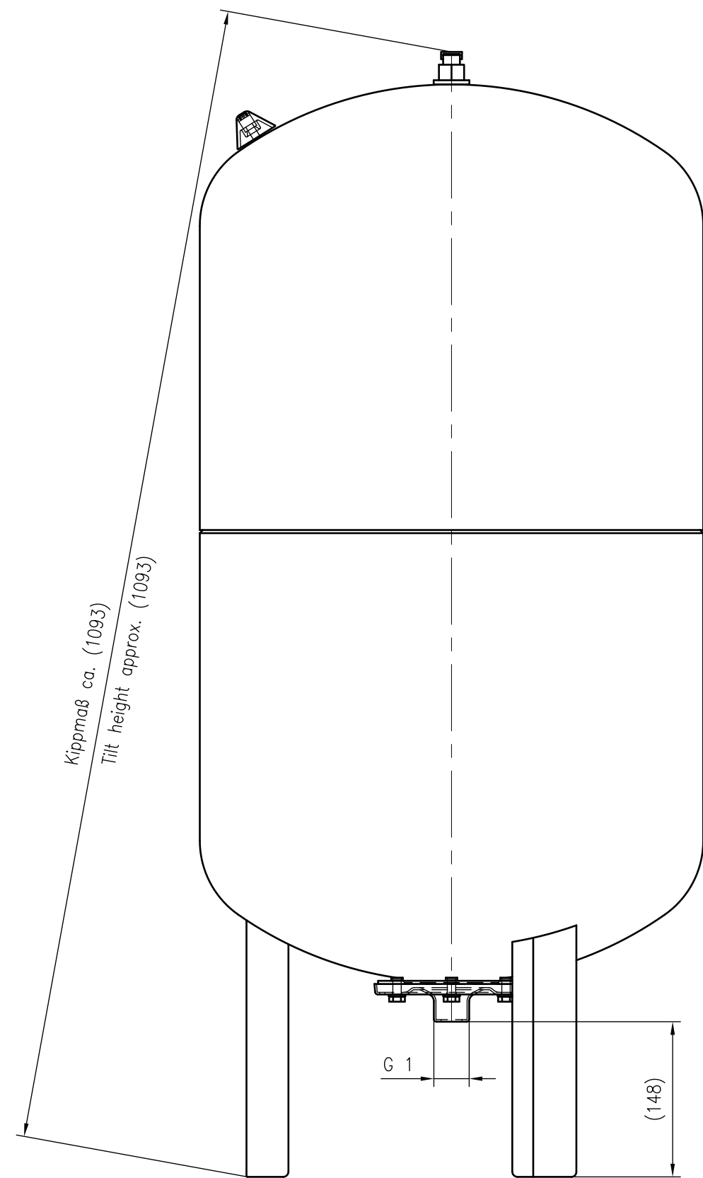
Side view
