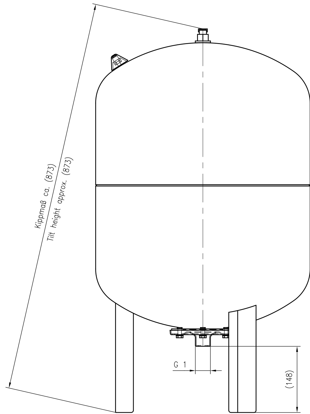
Side view
