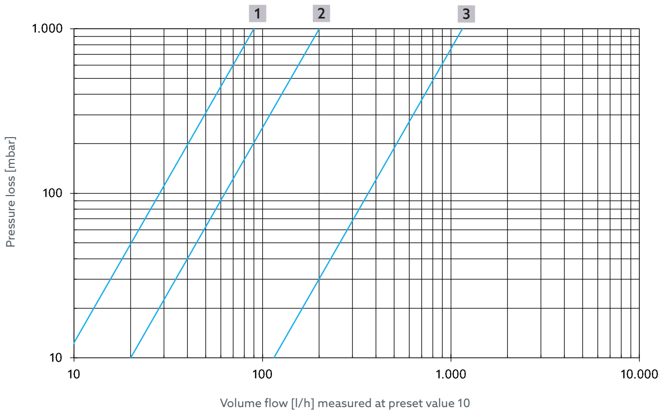
Fig. 17: Volume flow - Thermal control for item no. 4202504, 4202604, 4202704, 4202804
