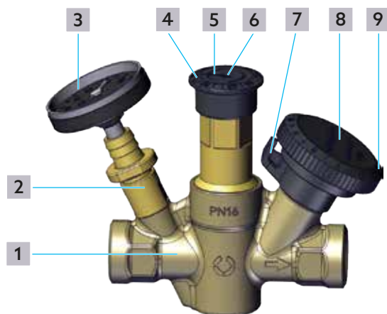
Fig. 1: Conception
