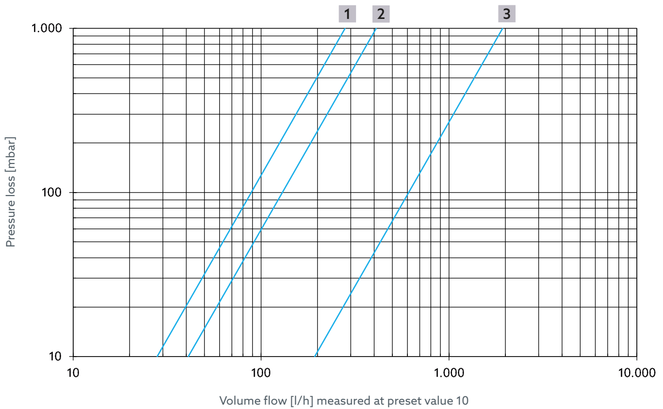
Fig. 19: Volume flow - Thermal control for item no. 4202506, 4202606, 4202706, 4202806
