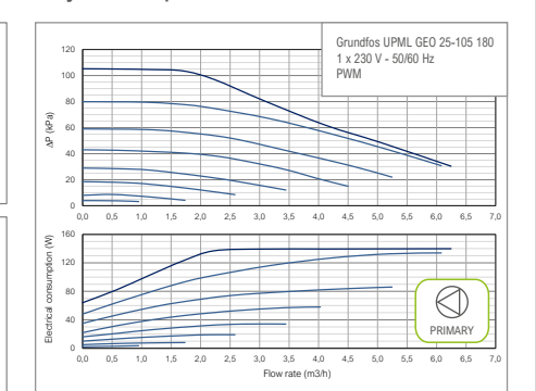
Hydraulic performance
