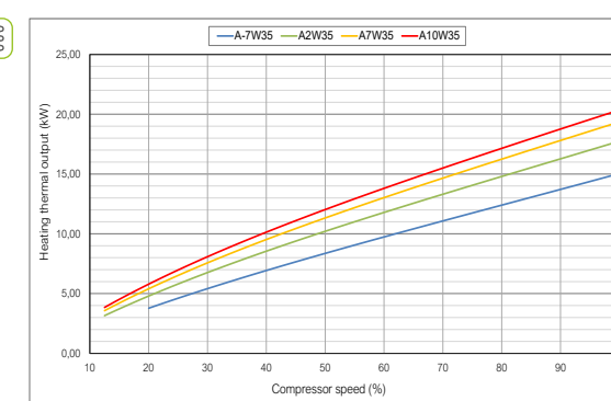
Thermal performance
