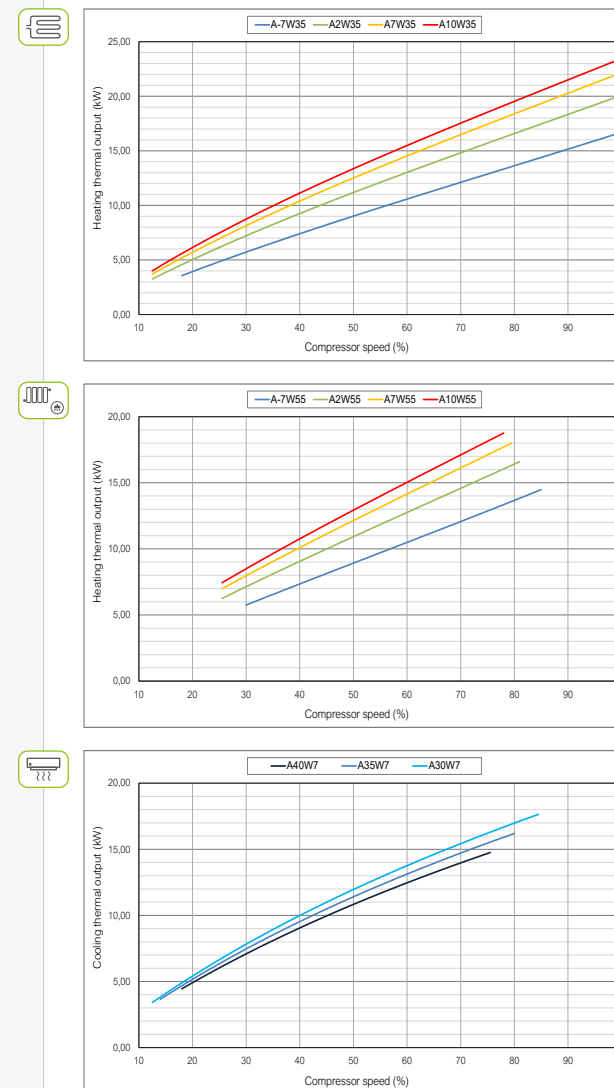
Thermal performance
