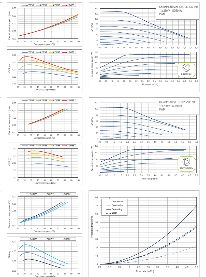
Hydraulic performance
