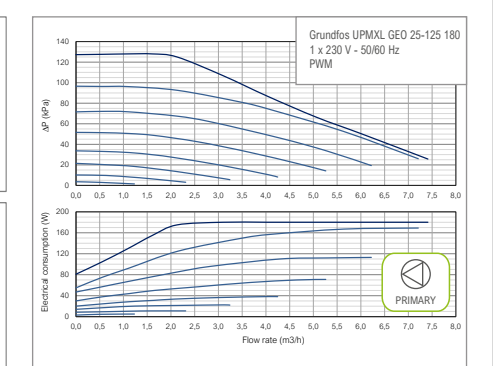
Hydraulic performance
